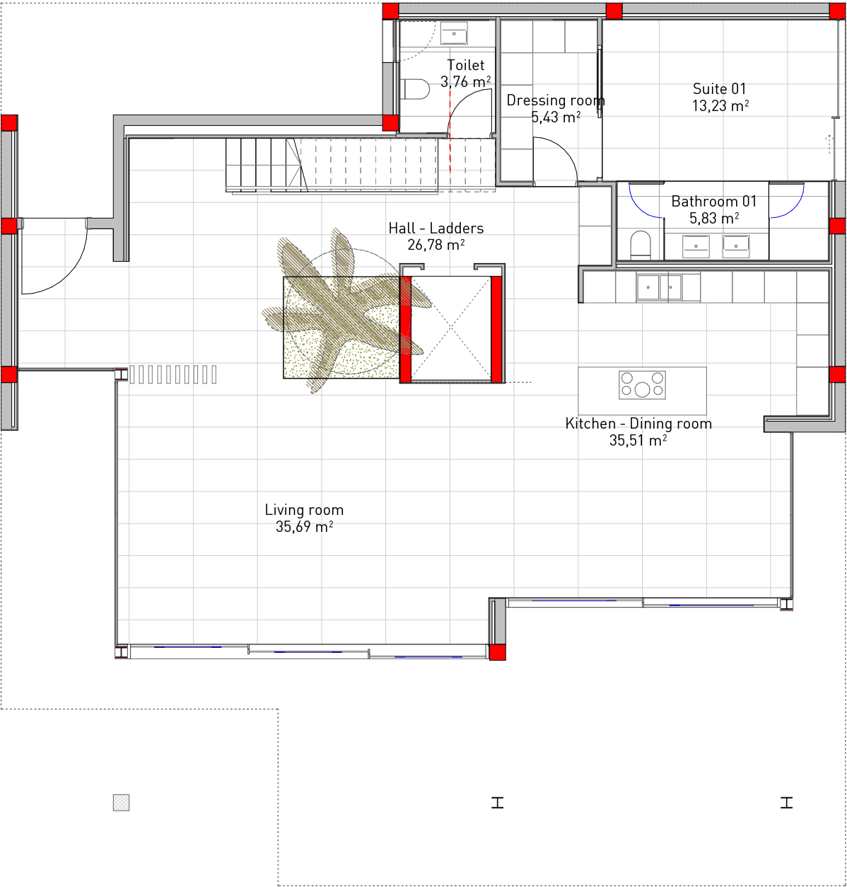
GROUND FLOOR - TIP A - 1:50
