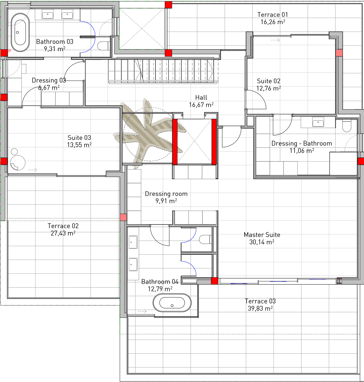
FIRST FLOOR - TIP A - 1:50
